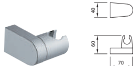
HABANA XTREME SOPORTE ARTICULADO Articulated holder Support douchette orientable
