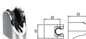
START SOPORTE ARTICULADO Articulated holder Support douchette orientable
