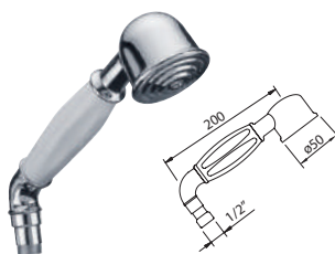
ANTIGONA | 1F | Ø50 mm DUCHA | Handset | Douchette
