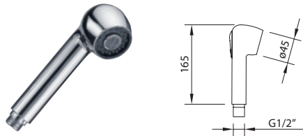
DUCHA Pull-out handshower for sink mixer | Douchette
